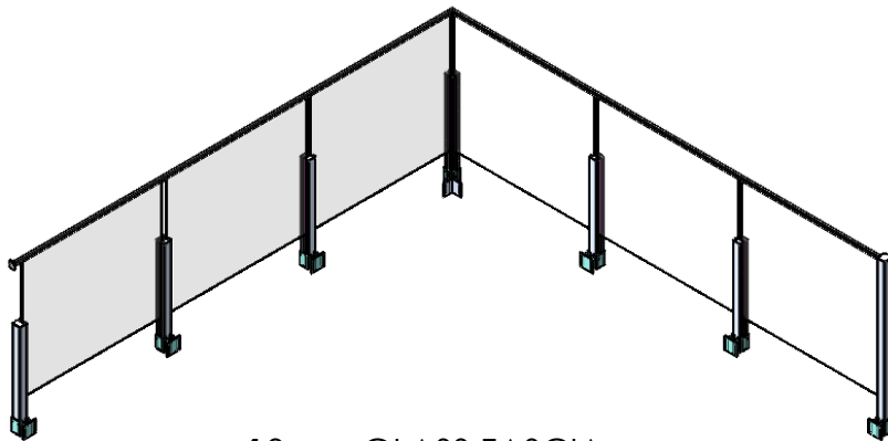
10mm GLASS FASCIA MOUNT RAILING
