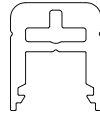
CenDek 10mm Glass Top Cap
